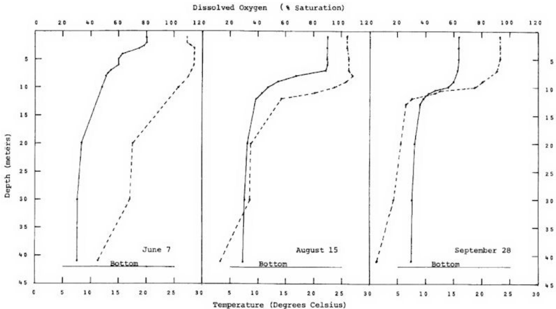
Figure 4: Temperature (—) and dissolved oxygen (---) profiles at Station 11 of Devil Lake, 1974.
