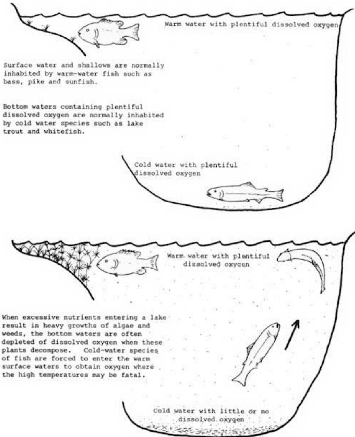
FIGURE A-1: Decomposition Of Plant Matter At The Lake Bottom Can Lead To Death Of Deep-water Fish Species.
