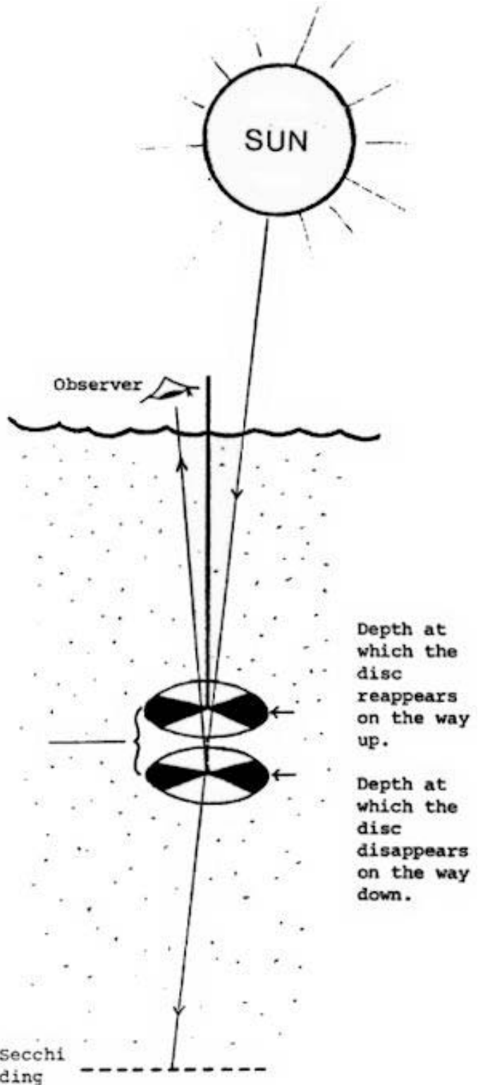
FIGURE 2: Use Of Secchi Disc To Determine Water Clarity.
