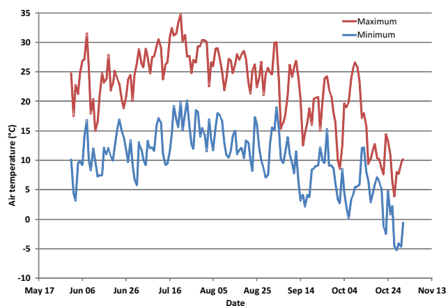
Figure 4. Daily air temperatures at GTI, summer 2011.
