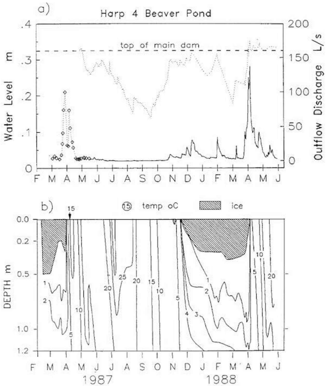
Figure 3. a) Water level and outflow discharge and b) temperature profile at site 1, Harp 4 beaver pond for March 1 1987 to May 31 1988.
