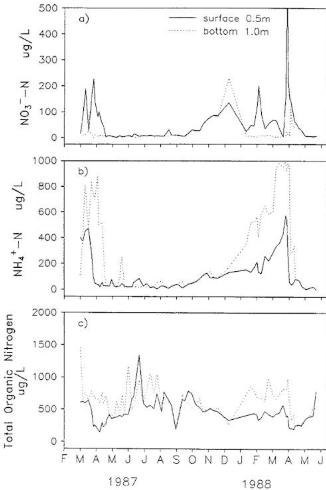
Figure 6. Seasonal variation in a) nitrate-nitrite nitrogen ( \text{NO}_3^- - \text{N} ), b) ammonium nitrogen ( \text{NH}_4^+ - \text{N} ) and c) total organic nitrogen (TON) concentrations of surface and bottom water at site 1 of Harp 4 beaver pond from March 1 1987 to May 31 1988.
