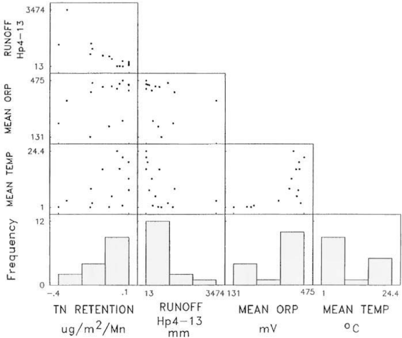
Figure 8. Pair-wise comparison of monthly total nitrogen (TN) retention with monthly runoff, mean redox potential and temperature for Harp 4 beaver pond for March 1987 to May 1988.
